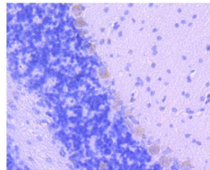
Fig. 2. Immunohistochemical analysis of paraffin-embedded rat cerebellum tissue using anti-LRP1 antibody. Counter stained with hematoxylin.
