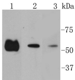
Fig. 1. Western blot analysis of Smad2 on different lysates using anti-Smad2 antibody at 1/1,000 dilution. Positive control: Lane 1: Hela; Lane 2: A431; Lane 3: PC12
