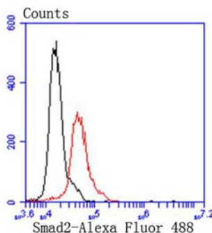
Fig. 3. Flow cytometric analysis of NIH/3T3 cells with Smad2 antibody at 1/50 dilution (red) compared with an unlabelled control (cells without incubation with primary antibody; black). Alexa Fluor 488-conjugated goat anti rabbit IgG was used as the secondary antibody.
